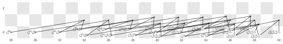
Figure 3.6: v_0^{-1} \text{Ext}_{E(2)*}(\Sigma^{28} \underline{\text{bu}}_7)
