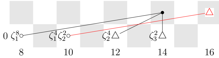
Figure 3.1: v_0^{-1} \text{Ext}_{E(2)*}(\Sigma^8 \underline{bu}_2)
