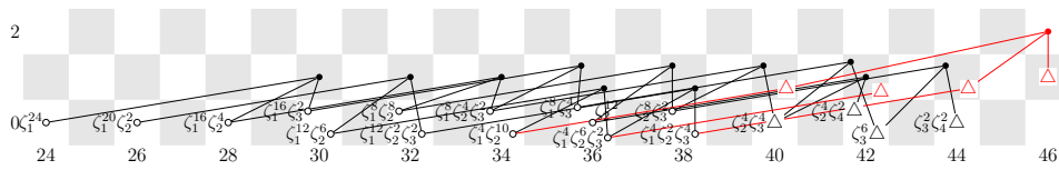
Figure 3.5: v_0^{-1} \text{Ext}_{E(2)*}(\Sigma^{24} \underline{bu}_6)
