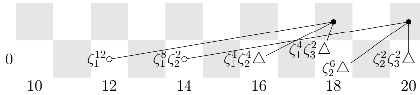
Figure 3.2: v_0^{-1} \text{Ext}_{E(2)*}(\Sigma^{12} \underline{bu}_3)
