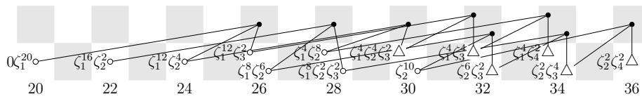
Figure 3.4: v_0^{-1} \text{Ext}_{E(2)*}(\Sigma^{20} \underline{bu}_5)
